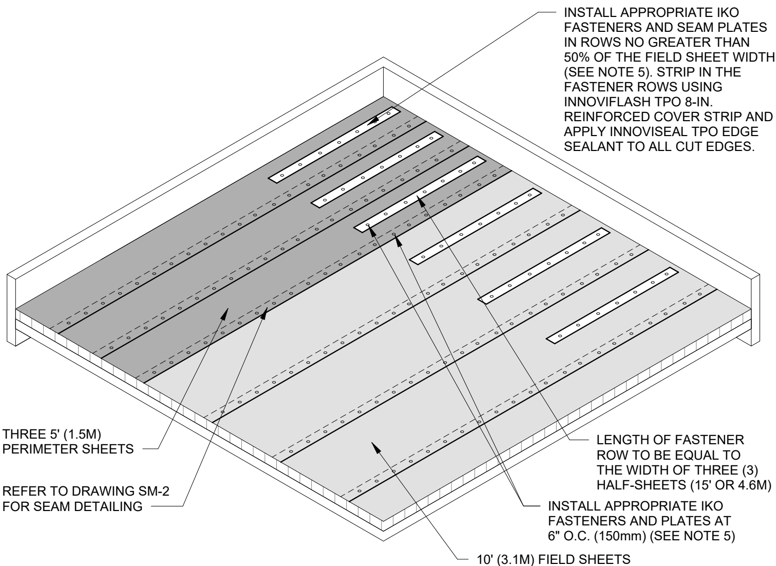
LAYOUT ATTACHMENT ML-10-3-6-F FOR 10' (3.1M) THERMOPLASTIC MEMBRANE PANELS
