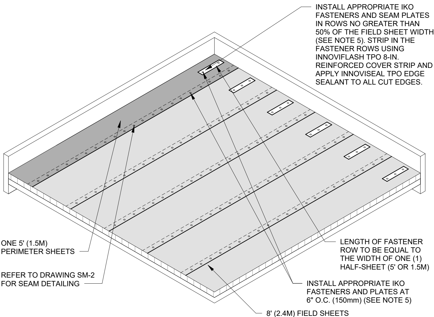
LAYOUT ATTACHMENT ML-8-1-6-F FOR 8' (2.44M) THERMOPLASTIC MEMBRANE PANELS
