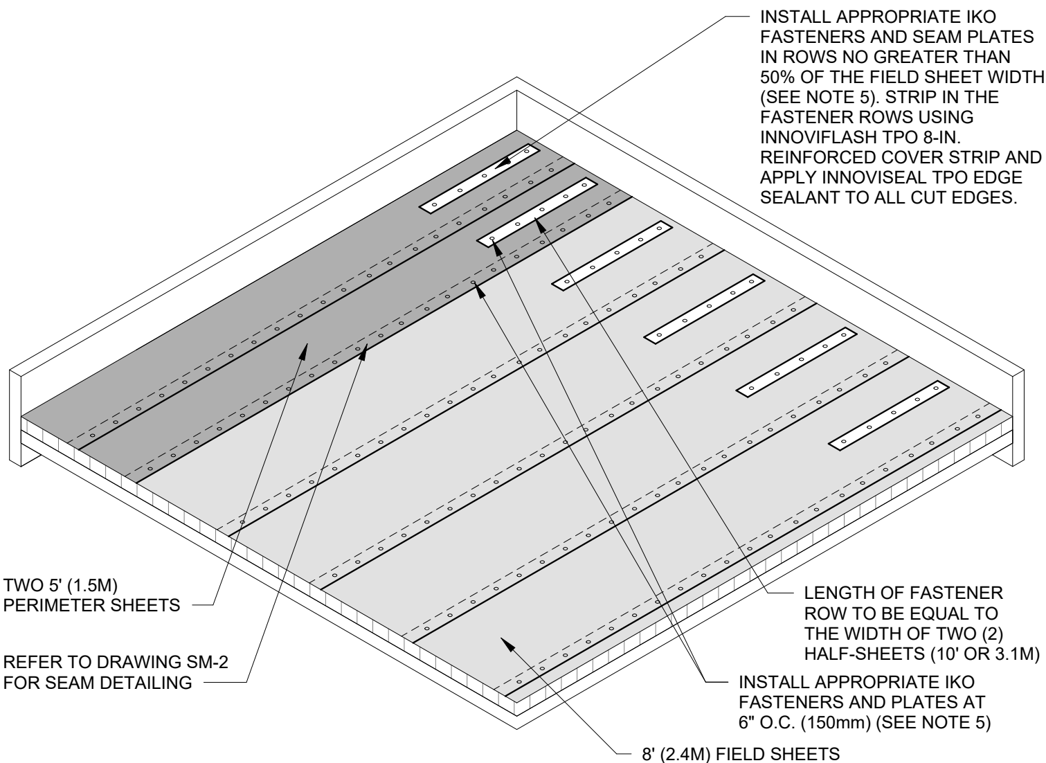
LAYOUT ATTACHMENT ML-8-2-6-F FOR 8' (2.44M) THERMOPLASTIC MEMBRANE PANELS
