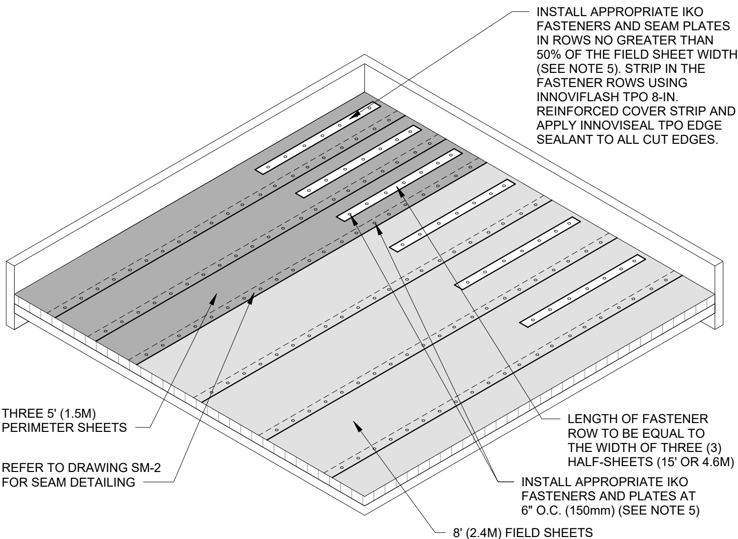
LAYOUT ATTACHMENT ML-8-3-6-F FOR 8' (2.44M) THERMOPLASTIC MEMBRANE PANELS
