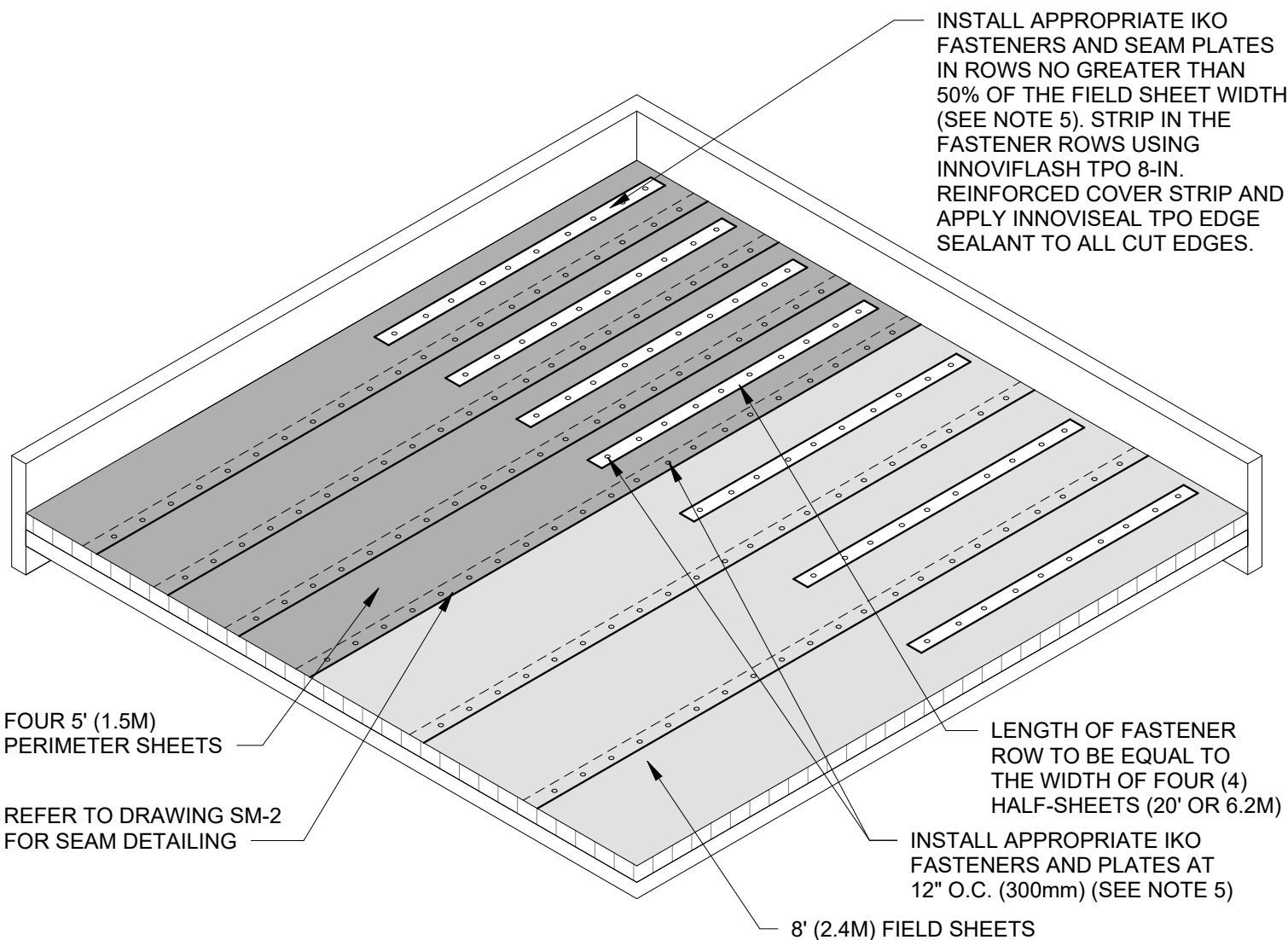
LAYOUT ATTACHMENT ML-8-4-12-F FOR 8' (2.44M) THERMOPLASTIC MEMBRANE PANELS
