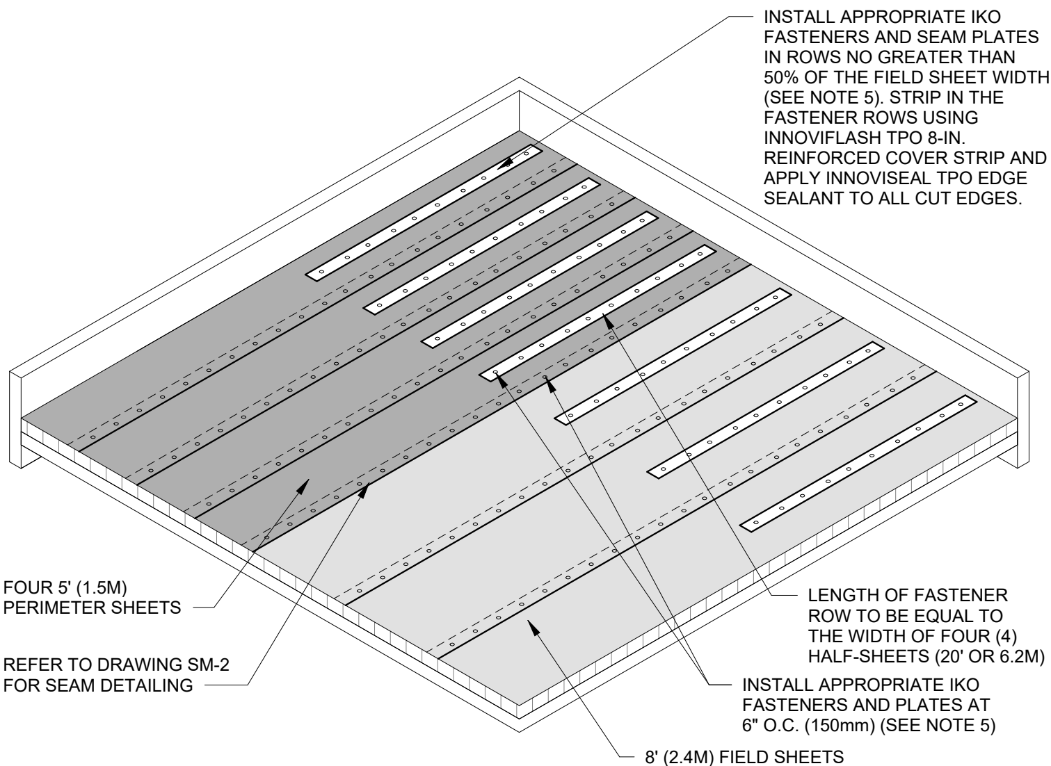
LAYOUT ATTACHMENT ML-8-4-6-F FOR 8' (2.44M) THERMOPLASTIC MEMBRANE PANELS
