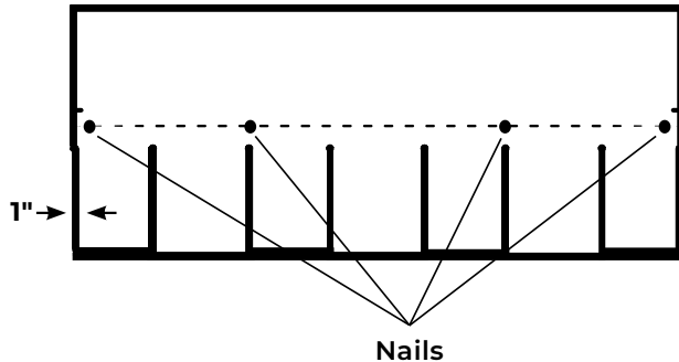
Standard Application Requires 4 Nails
