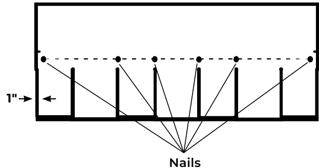
Steep Slope/High Wind Applications Requires 6 Nails
